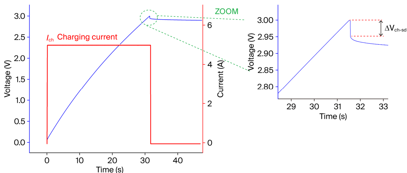
Figure 6. Charge and self-discharge (ch-sd) of a 60 F SC. ESR was calculated as the inverse ratio between the charging current I_{ch} and the voltage drop \Delta V_{ch\_sd} , which appears when the charging current stops.
