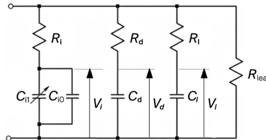
Figure 2. Three-branch electrical circuit model of an SC.
