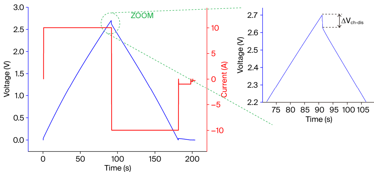
Figure 9. Charge at cc up to the rated voltage and immediate discharge at cc for a 400 F SC. Charge and discharge (ch-dis) are supplied with the same current. In the figures the blue line refers to the terminal voltage at the and the red line refers to the current.
