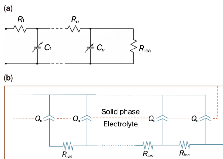
Figure 1. (a) TLM circuit model; (b) simplified form of the transmission line model for porous electrodes [36].
