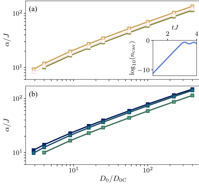
FIG. 5. One-dimensional cavity-atoms simulations. (a) Growth rate \alpha in units of the hopping amplitude J as a function of D_0/D_{0C} , obtained from the numerical simulations of Eqs. (E1) and (E2) for fermionic atoms, Eq. (E3), with on-site interaction strengths U/J : 0 (—), 4 (—), 16 (—). The inset shows the exponential growth of the intracavity photon number n_{\text{cav}} for a quench to D_0/D_{0C} = 4 and U/J = 4 as a function of time t . (b) Growth rates for bosonic atoms, Eq. (E4), with U/J : 0.25 (—), 4 (—), \infty (—). The parameters used for panels (a) and (b) are \hbar\tilde{\Delta}_c/J = 200 and \hbar\kappa/J = 3.75 , considering a similar separation of scales as in the experiment. The simulations were performed for L = 48 sites and an atomic filling N/L = 0.375 . The filling was chosen not to be commensurate with the potential induced by the cavity.
