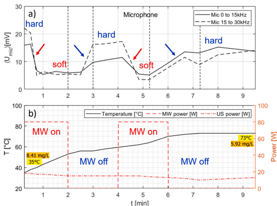
Fig. 10. Measurement time traces for slightly pre-heated water under continuous US irradiation and with two times 2 min, 80 W MW on and off switching. (a) Air microphone integrated spectrum from 0 to 15 kHz (continuous line) and 15 to 30 kHz (broken line); (b) temperature readout (continuous line, left ordinate) and powers (right ordinate) of MW (dashed) and US horn (dash-dotted). Initial and final temperature and oxygen concentrations are indicated. The red arrows show the transitions from hard to soft cavitation, the blue arrows the return to hard cavitation. Initial and final temperature and oxygen concentrations are indicated. Black dashed vertical lines in (a) indicate the time instances where sample spectra are shown in the Appendix, Fig. A.17 .
