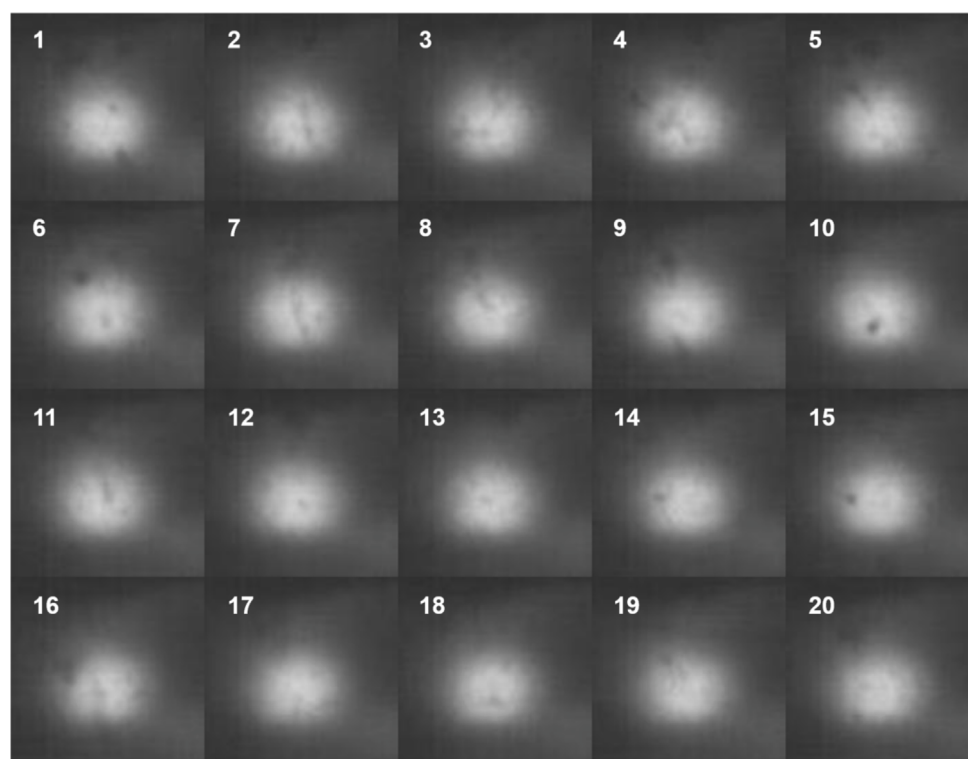
Fig. B.20. Frames from a high-speed recording series of hard cavitation in setup III. Frame width 4.4 mm, interframe time 1 ms, exposure time 1 ms. ((Link to the movie “HardCavitation_in_MW.avi”)).
