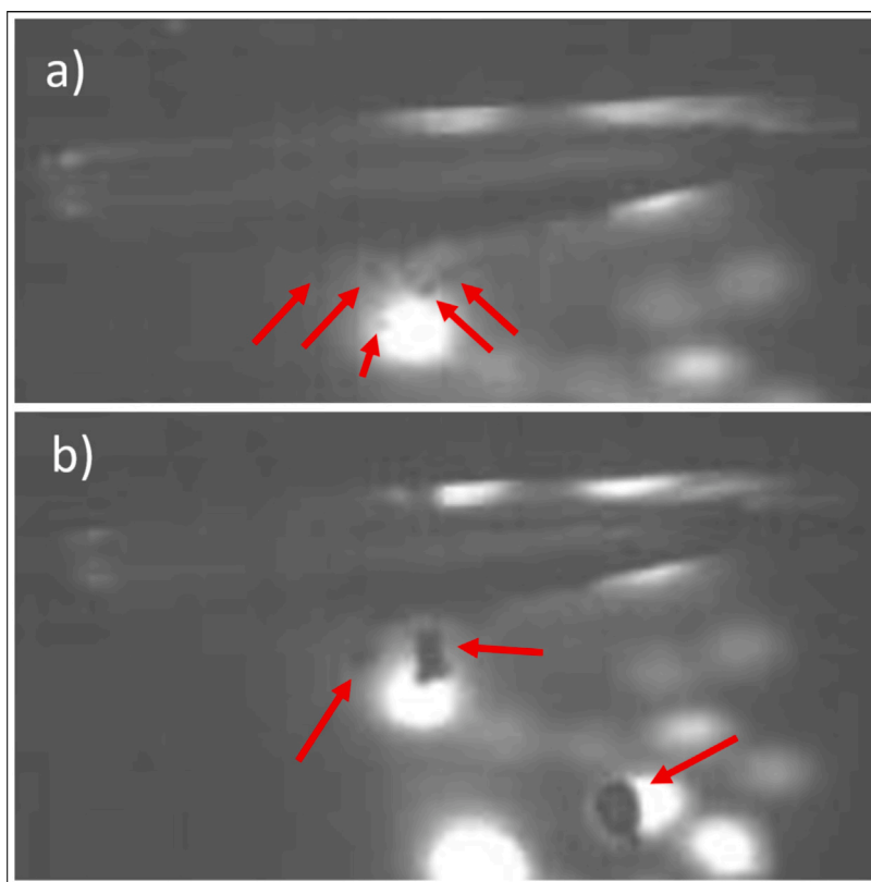
Fig. 12. Optical recordings in setup III from within the MW oven for (a) hard and (b) soft cavitation states. Frame width about 20 mm, the horn tip is visible in the top. The arrows mark cavitation bubbles in the low contrast images. Similarities with the recordings from setup II are striking, see Fig. 5.
