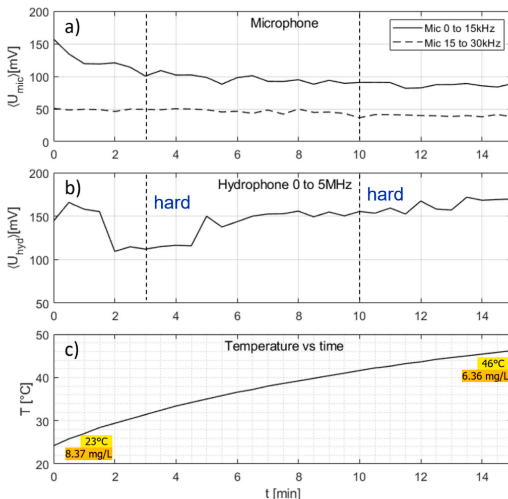
Fig. 7. Measurement time traces for room temperature water (net heating) under continuous 30 W US application alone (no MW). (a) Air microphone integrated spectrum from 0 to 15 kHz (continuous line) and 15 to 30 kHz (broken line); (b) hydrophone integrated spectrum from 0 to 5 MHz; (c) temperature readout. Initial and final temperatures and oxygen concentrations are indicated. The cavimeter was not available for this run, but high levels of microphone and hydrophone report hard cavitation throughout. Black dashed vertical lines indicate the time instances where sample spectra are shown in Appendix A, Fig. A.15 .
