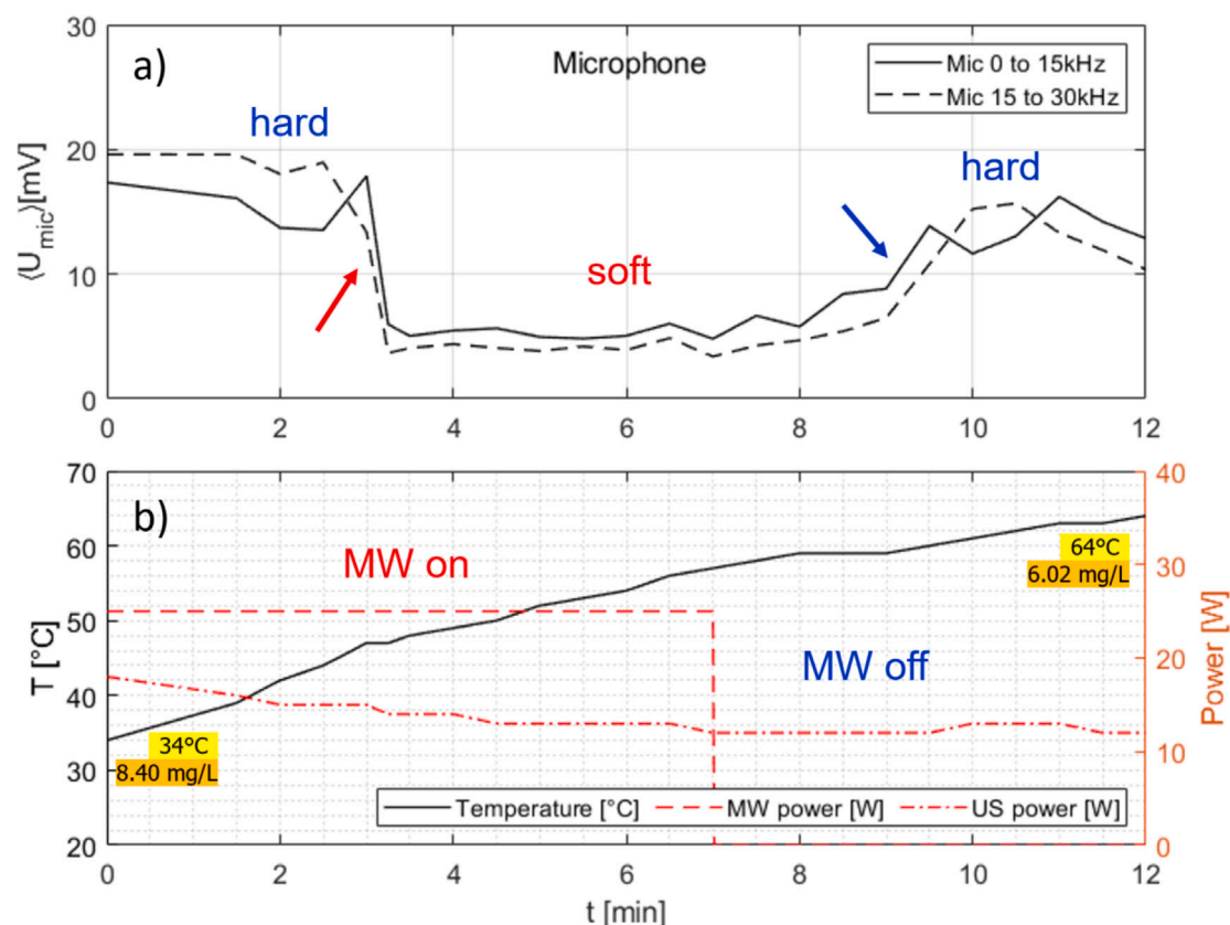
Fig. 9. Measurement time traces for room temperature water under continuous US irradiation and additional MW application of 25 W, switched off after 7 min. (a) Air microphone integrated spectrum from 0 to 15 kHz (continuous line) and 15 to 30 kHz (broken line); (b) temperature readout (continuous line, left ordinate) and powers (right ordinate) of MW (dashed) and US horn (dash-dotted). Initial and final temperature and oxygen concentrations are indicated. The red arrow shows the transition from hard to soft cavitation, the blue arrow the return to hard cavitation.
