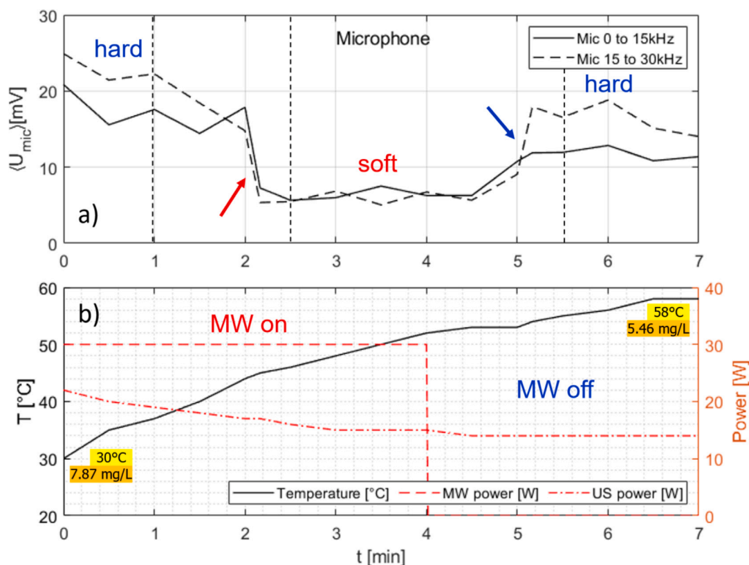
Fig. 8. Measurement time traces for room temperature water under continuous US irradiation and additional MW application of 30 W, switched off after 4 min. (a) Air microphone integrated spectrum from 0 to 15 kHz (continuous line) and 15 to 30 kHz (broken line); (b) temperature readout (continuous line, left ordinate) and powers of MW (dashed) and of US horn (dash-dotted). Powers refer to right ordinate. Initial and final temperatures and oxygen concentrations are indicated. The red arrow shows the transition from hard to soft cavitation, the blue arrow the return to hard cavitation. Sample spectra are given in Appendix A, Fig. A.16 , for the time instances marked by black dashed vertical lines in (a).
