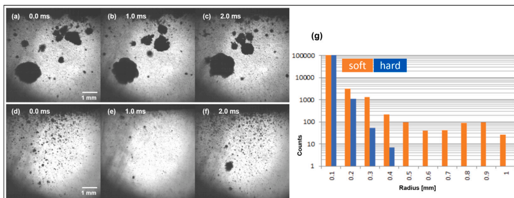
Fig. 5. Left: Soft cavitation and hard cavitation in an experiment in setup II, similar to the run presented in Fig. 6, but US power 45 W. Top movie frames (a), (b), (c): soft cavitation; bottom movie frames (d), (e), (f): hard cavitation (times and scales indicated). The disappearance of many small bubbles between frames (d) and (e) highlights their oscillation with a strong collapse, a feature not observed for the larger bubbles in (a), (b). Longer sequences are given in Appendix B, and both movies are provided as Supplementary Material. (g): Bubble radius statistics evaluated over 2000 subsequent frames from the same high-speed movies. Orange (left) histogram bars correspond to the soft, blue (right) bars to the hard cavitation state. Every frame was evaluated, and thus bubbles at different expansion or collapse state are included. Still, a clear difference is obvious. Bubble radii larger than about 0.5 mm were not observed in the hard regime, but were frequent in the soft regime.
