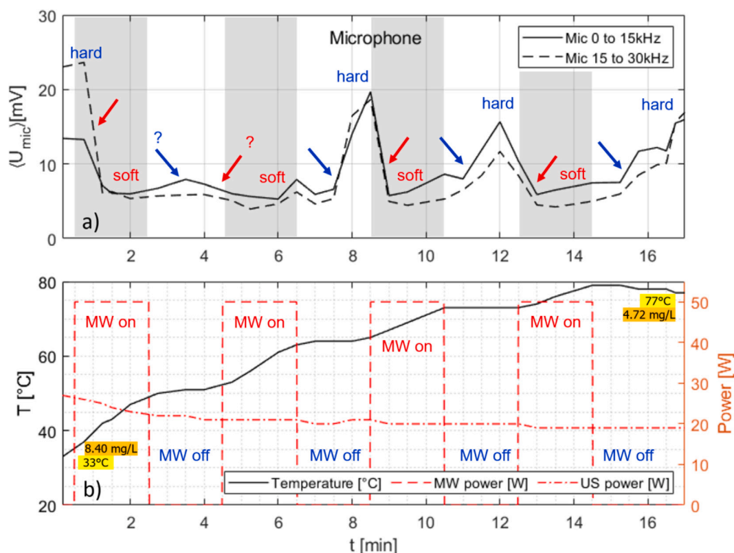
Fig. 11. Measurement time traces for slightly pre-heated water under continuous US irradiation and with alternating 2 min, 50 W MW on and off switching. (a) Air microphone integrated spectrum from 0 to 15 kHz (continuous line) and 15 to 30 kHz (broken line); (b) temperature readout (continuous line, left ordinate) and powers (right ordinate) of MW (dashed) and US horn (dash-dotted). Initial and final temperature and oxygen concentrations are indicated. The red arrows show the transitions from hard to soft cavitation, the blue arrows show the return to hard cavitation. The acoustic signal change during the first MW off phase is weak, so a switch to hard cavitation and back is doubtful (marked by “?”). In the other intervals, rather clear transitions occurred. For clarity, the MW episodes are shaded in (a).
