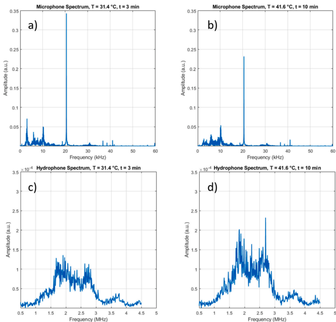
Fig. A.15. Sample spectra of two time instants marked in Fig. 7, room temperature water sonicated continuously. The actual temperature and sample time of the spectral recordings is denoted above the plots. (a) and (b) show microphone spectra up to 60 kHz, both indicating an inertial cavitation regime by a rather high noise floor around and below 10 kHz. Simultaneously measured hydrophone spectra from 0.5 to 5 MHz are shown in (c) and (d). They contain as well a significant broadband noise level.
