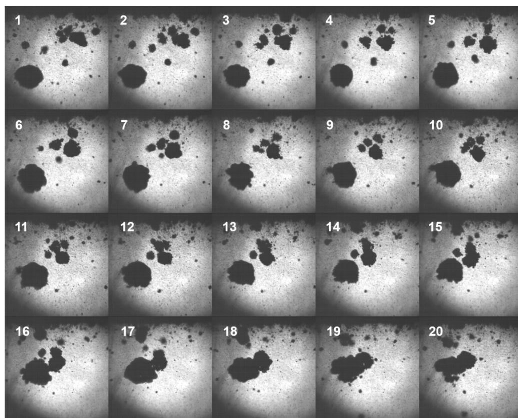
Fig. B.18. Frames from a high-speed recording series of soft cavitation in setup II. Frame width 6 mm, interframe time 0.2 ms, exposure time 20 \mu s. The movie can be found in the Supplementary Material ((Link to the movie "SoftCavitation.avi")).
