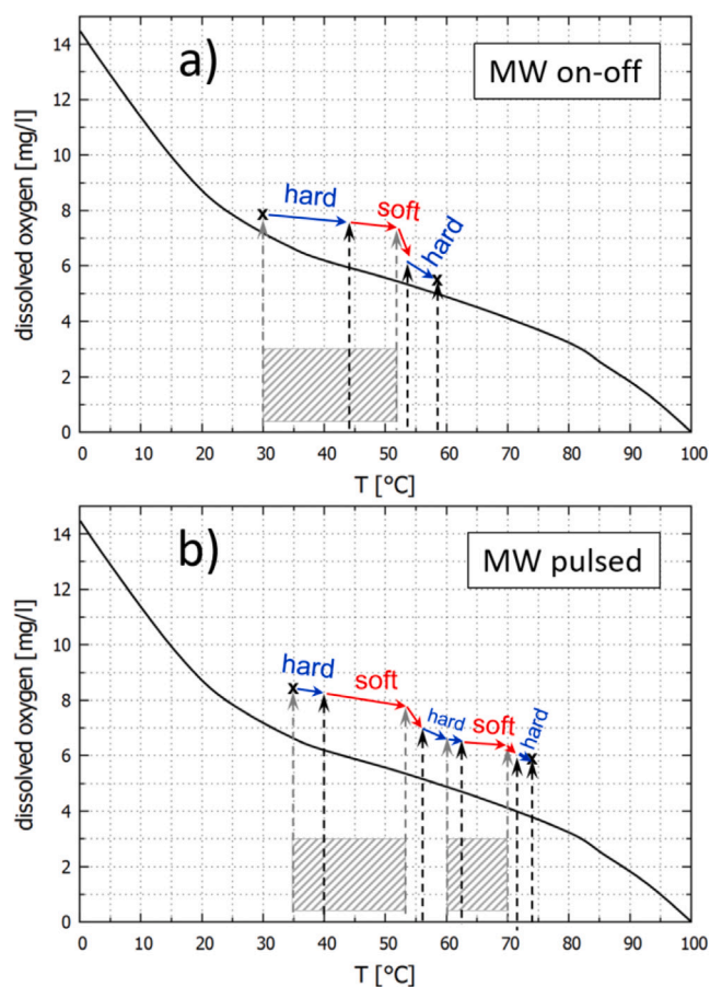
Fig. 14. Progression of the experiments in the state space of temperature and dissolved oxygen concentration: (a) Room temperature water, US + MW on-off, Fig. 8. (b) Slightly pre-heated water, US + MW pulsed 2 min on-off, Fig. 10. The black reference curve represents the equilibrium saturation of oxygen in water under air atmosphere at standard conditions, as obtained from [37]. Red arrows mark soft cavitation, blue arrows denote hard cavitation. Initial and end points (crosses) and transition temperatures (positions of vertical dashed arrows) were measured, intermediate progression is conjectured. The gray shaded regions indicate the phases of MW on.
