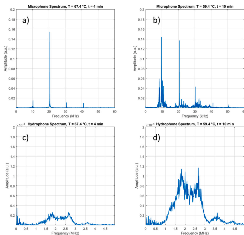
Fig. 4. Illustration of acoustic spectra for gassy vs. inertial cavitation, taken from the experiment discussed below in Fig. 6. Left frames: (a) air microphone and (c) hydrophone spectra for gassy cavitation (recorded after 4 min of the run, at T = 67.4\text{ }^{\circ}\text{C} ). Right frames: (b) air microphone and (d) hydrophone spectra for inertial cavitation (recorded after 10 min of the run, at T = 59.4\text{ }^{\circ}\text{C} ).
