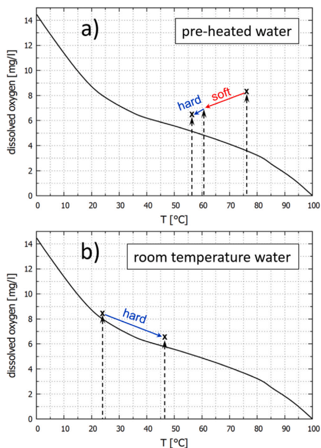
Fig. 13. Progression of the experiments in the state space of temperature and dissolved oxygen concentration: (a) Pre-heated water, only US, Fig. 6. (b) Room temperature water, only US, Fig. 7. The black reference curve represents the equilibrium saturation of oxygen in water under air atmosphere at standard conditions, as obtained from [37]. Red arrows mark soft cavitation, blue arrows denote hard cavitation. Initial and end points (crosses) and transition temperatures (positions of vertical dashed arrows) were measured, intermediate progression is conjectured.
