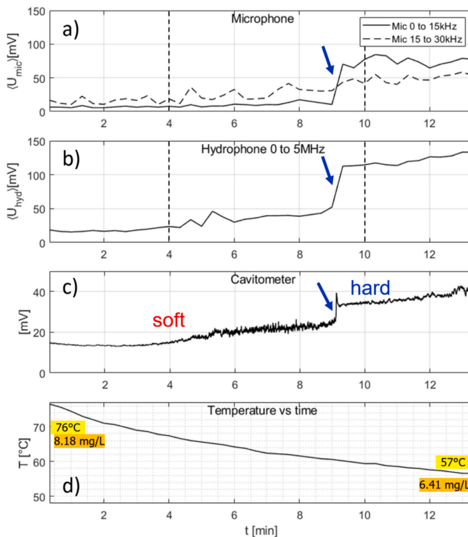
Fig. 6. Measurement time traces for pre-heated water (net cooling) under continuous 30 W US application alone (no MW). (a) Air microphone integrated spectrum from 0 to 15 kHz (continuous line) and 15 to 30 kHz (broken line); (b) hydrophone integrated spectrum from 0 to 5 MHz; (c) cavitometer readout; (d) temperature readout. Initial and final temperatures and oxygen concentrations are indicated. Blue arrows mark the transition from soft to hard cavitation. The black dashed vertical lines in (a) and (b) indicate the time instances when the spectra in Fig. 4 had been recorded.
