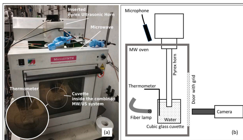
Fig. 3. Experimental setup III: Photograph (a) and schematic (b) of the custom MW oven device with the Pyrex horn inserted from top. The cuvette (see magnified inset) was placed inside the combined MW/US system with a special fiber optical thermometer that was used to record the water temperature over time. A fiber optic light source was used to back-light the cuvette. The camera was placed just outside the glass window. Due to the protective mesh behind the glass window, the field of view that the camera could record was hampered.
