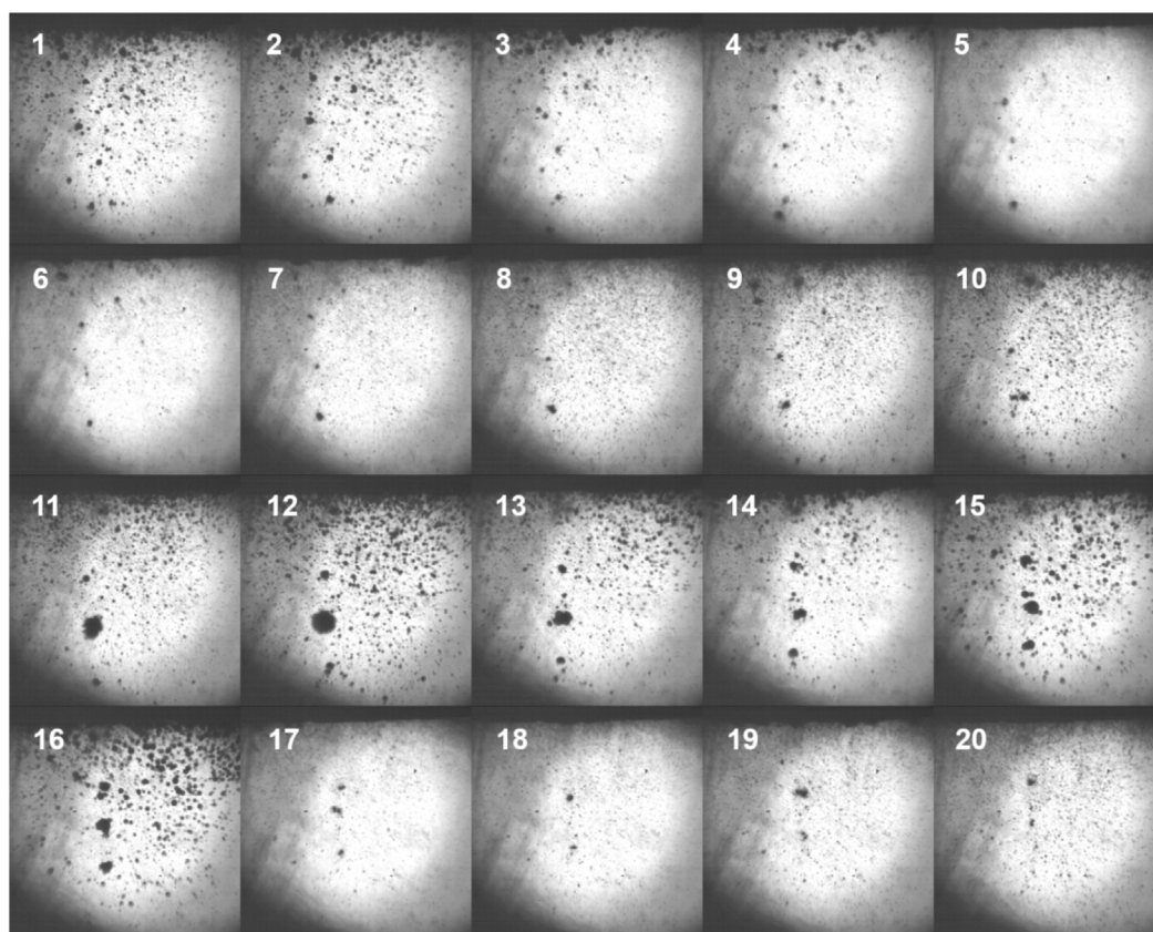
Fig. B.19. Frames from a high-speed recording series of hard cavitation in setup II. Frame width 6 mm, interframe time 0.2 ms, exposure time 20 \mu s. The movie can be found in the Supplementary Material ((Link to the movie “HardCavitation.avi”)).
