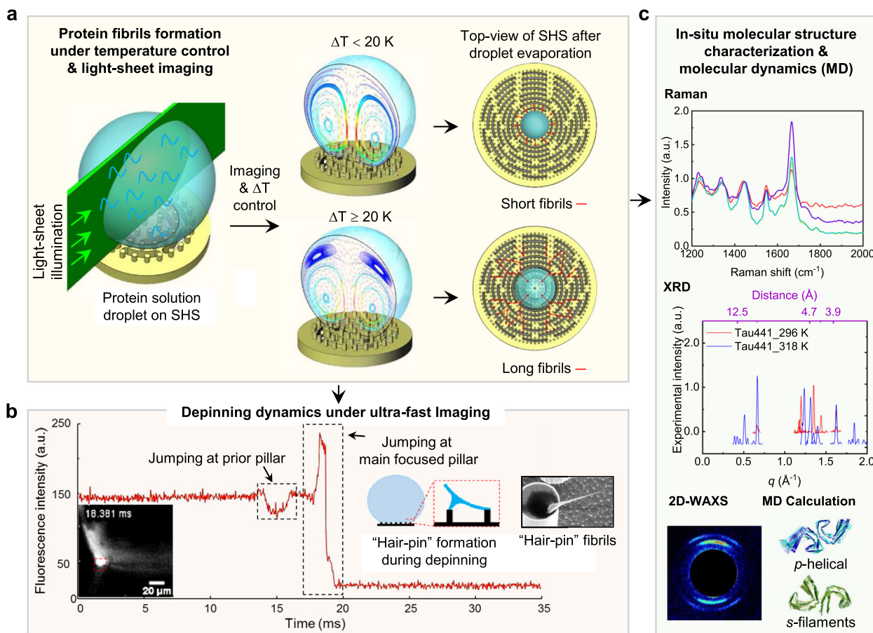
Fig. 1 Scheme of the whole process from protein fibril formation in droplet with confined convective flow field control and study of droplet contact line depinning dynamics to protein fibrils molecular structure characterizations. a Protein fibrils formation with temperature gradient ( \Delta T ) controlled confined convective flow field in droplet on SHS. b Droplet contact line depinning dynamics study with ultra-fast imaging. c In situ molecular structure characterizations of protein fibrils with Raman, XRD, 2D-WAXS, and molecular dynamics (MD) calculation.
