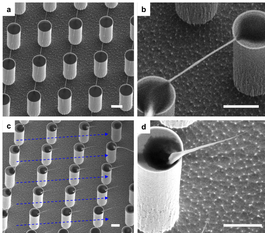
Fig. 3 SEM images of final amyloid fibril depositions on SHS after the drop evaporation. a, b Suspended and stretched amyloid fibrils with different size. c, d “Hair-pin” morphology formed on the top of micro-pillars. Scale bars are 5 \mu\text{m} .
