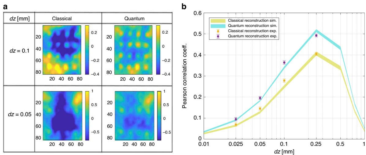
Fig. 6 Single-frame reconstruction of the squares pattern. a Examples of classical and quantum reconstructions of the sample with squares in Fig. 2 (right-hand side) for two different defocussing distances. b Pearson correlation coefficient between the reconstructed phase image by a single intensity frame and the reference image as a function of the defocussing
