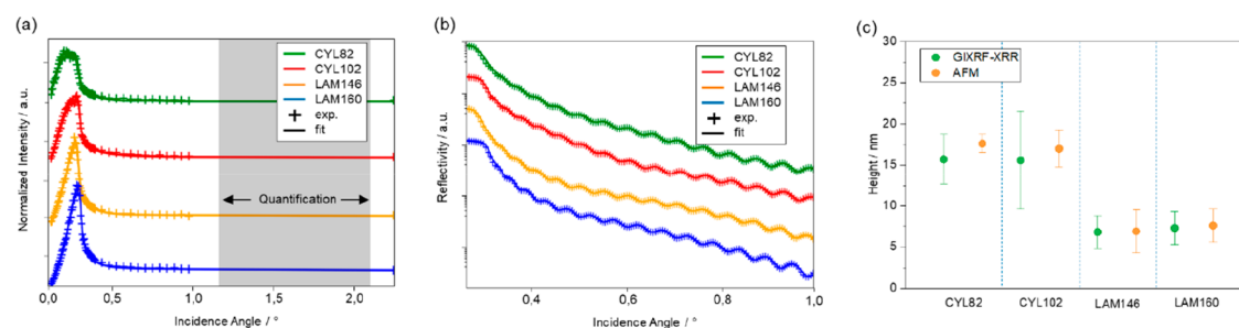
Figure 3. (a) Ti–K GIXRF spectra for the infiltrated TiO 2 nanostructures measured at FCM beamline with a 6 keV incident beam energy (the data in the angular range above the critical angle for total external reflection highlighted in gray, can be used for the quantification of the element of interest) and (b) relative reflectivity curves. (c) Comparison of the infiltrated TiO 2 height values obtained by AFM measurements and GIXRF-XRR modeling. Confidence intervals ( 1\sigma ) of the GIXRF-XRR hybrid model are derived from Markov chain Monte Carlo analysis. 58
