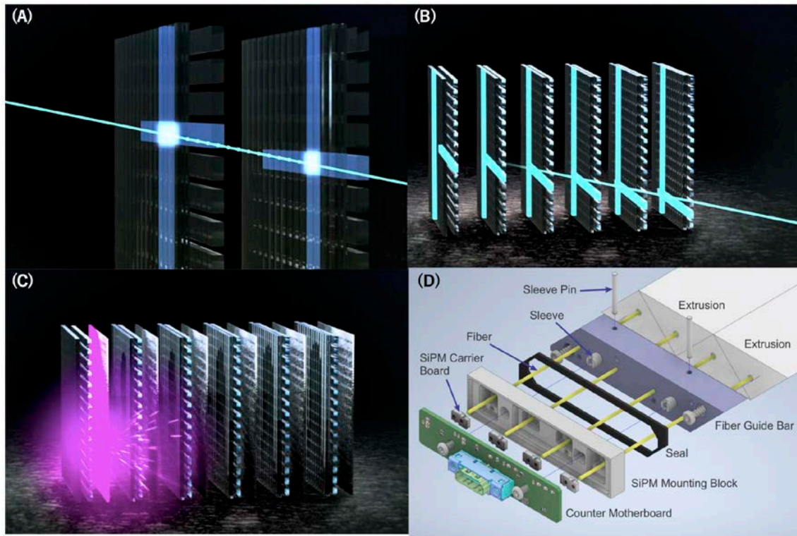
Fig. 2| (A) X-Y position from detector, (B) Muon tracker with multiple PSDs, (C) Illustration of rejection of electromagnetic components via Multiple-Coulomb Scattering, (D) Quad-counter| Diagram of Quad-counter showing the triangular scintillator extrusion, wavelength-shifting fiber readout and SiPM photon detector 28 .
