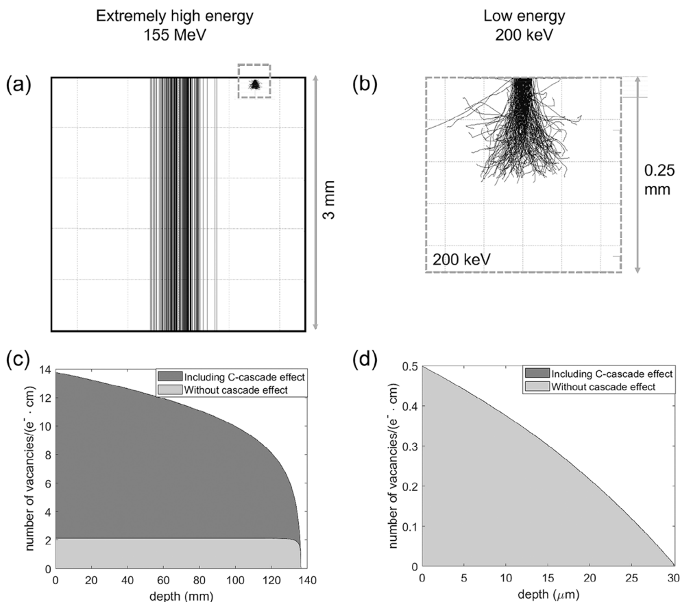
Figure 1. a,b) Trajectories of 200 electrons in diamond, simulated using CASINO software. a) 155 MeV electron irradiation, 500 μm beam diameter. b) 200 keV electron irradiation, 15 μm beam diameter. c,d) Simulation of the number of vacancies per centimeter depth generated by 1 accelerated electron at c) 155 MeV energy and d) 200 keV energy. The contribution of the initial recoiled atoms (filled light gray) and the secondary cascade process (filled dark gray) are highlighted. Note the different axes limits in the two cases.
