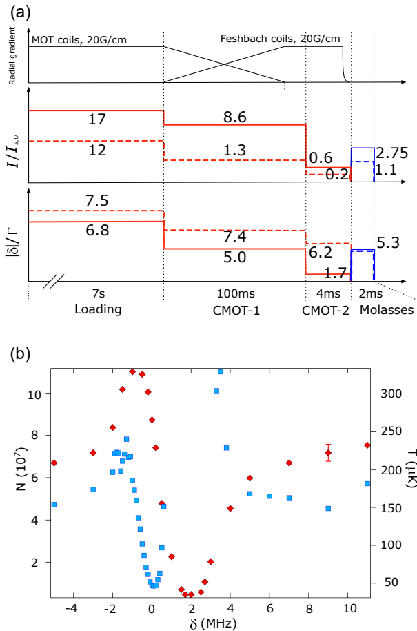
FIG. 4. (a) Sketch of the experimental routine employed to produce cold clouds of ^6\text{Li} atoms in our experiment. For each stage, red (blue) solid and dashed lines indicate the parameters exploited for D_2 ( D_1 ) cooling and repumper lights, respectively. The transfer from the MOT coils to the Feshbach coils quadrupole is also shown by the black solid lines. (b) Temperature (right axis, blue squares) and atom number (left axis, red diamonds) as a function of the relative detuning \delta of the D_1 repumper and cooling lights, recorded after 2 ms of gray molasses. At the Raman condition, \delta = 0 , a minimum temperature of 45(5) \mu\text{K} is obtained, with a cooled fraction N/N_0 \sim 75\% . For this measurement, the total cooling and repumper peak intensities were fixed to the optimum values I_{cool} = 2.75 I_{S,Li} and I_{rep} \sim 0.4 I_{cool} , respectively.
