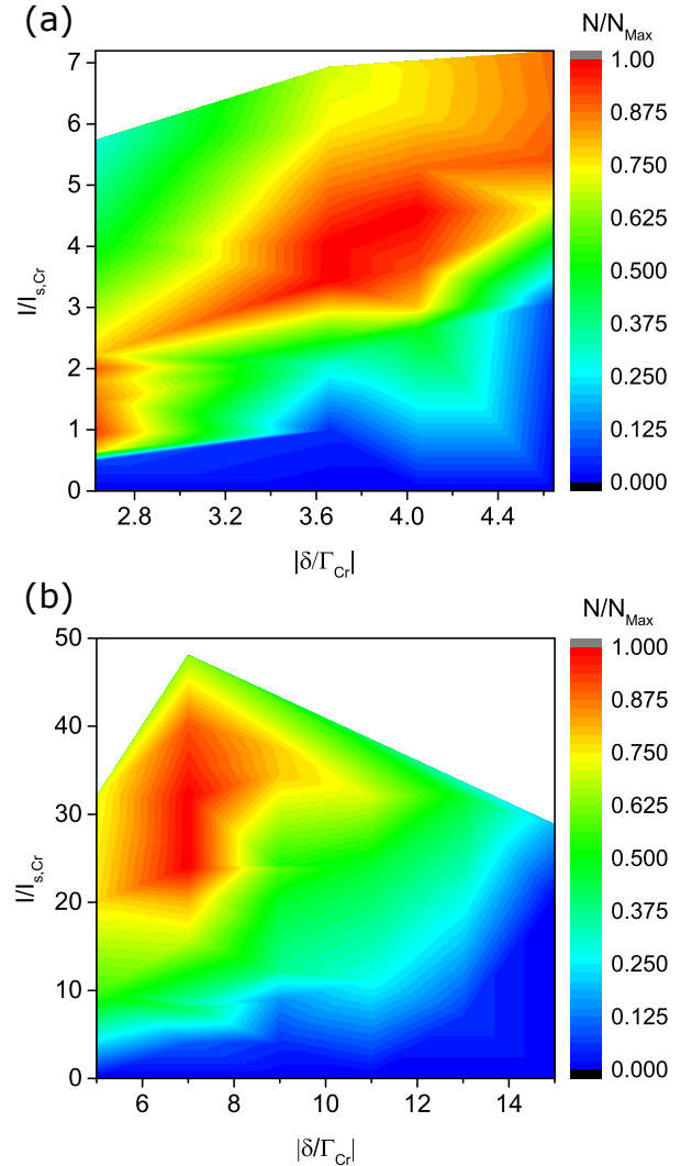
FIG. 5. (a) Steady-state MOT population, rescaled to its optimum value, as a function of both the normalized single-beam peak intensity I/I_{S,Cr} and the detuning \delta/\Gamma_{Cr} of the cooling light, see color code on the right. This measurement employs a radial MOT gradient of 12.6\text{ G/cm} , and a ZS beam intensity (detuning) of 32 I_{S,Cr} ( -7\Gamma_{Cr} ). (b) Same as panel (a) but for the ZS cooling beam parameters. The given ZS beam intensity corresponds to the one estimated at the MOT region. For this measurement, the single MOT beam peak intensity (detuning) is set to 3.5 I/I_{S,Cr} ( -3.5\Gamma_{Cr} ).
