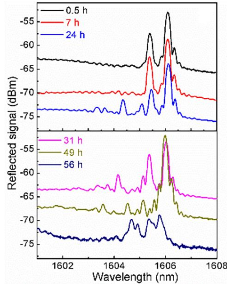
Fig. 11. Reflected signal evolution of an 1^\circ tilted FBG immersed in PBS solution for up to 56 h. The baseline of the different spectra has been adjusted vertically to assist visualization. Adapted from [26] under the Creative Common license CC BY.
