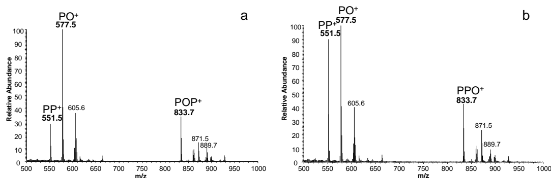
Figure 2. Full mass spectra of isobaric positional isomers POP (palmitoyl-oleoyl-palmitoyl glycerol) (a) and PPO (palmitoyl-palmitoyl-oleoyl glycerol) (b) showing the specificity of thermal fragmentation mechanism.
