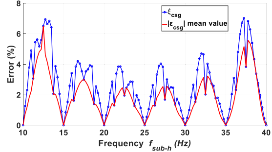
Fig. 4. Mean absolute value and maximum absolute value ( \xi_{csg} ) of \varepsilon_{csg} , introduced by the signal processing in the measurement of Y_{csg} , versus the generated subharmonic frequency.
