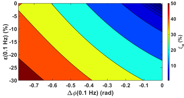
Fig. 13. Maximum value of \zeta_g versus IT ratio and phase errors at 0.1 \text{ Hz} .
