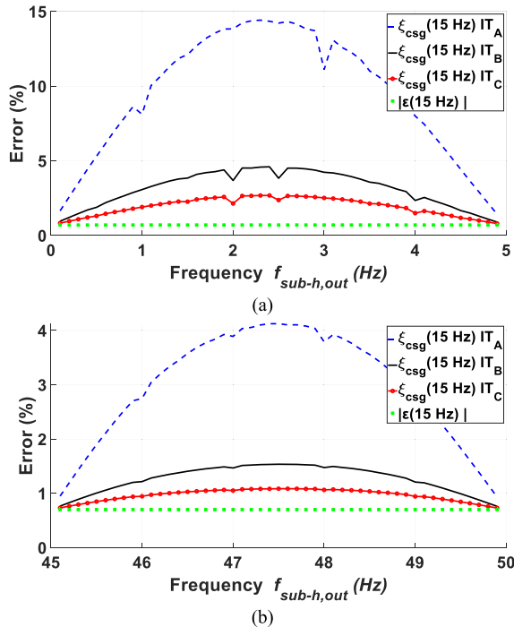
Fig. 11. Maximum error ( \xi_{\text{csg}} ) introduced by linear ITs, with different phase error responses, when signals composed of tones with f_{\text{sub-h}} equal to 15 Hz and f_{\text{sub-h,out}} in (a) [0.1, 4.9] Hz range and (b) [45.1, 49.9] Hz range are analyzed.
