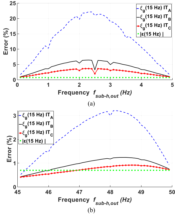
Fig. 10. Maximum error ( \xi_g ) introduced by linear ITs, with different phase error responses, when signals composed of tones with f_{\text{sub-h}} equal to 15 Hz and f_{\text{sub-h,out}} in (a) [0.1, 4.9] Hz range and (b) [45.1, 49.9] Hz range are analyzed.
