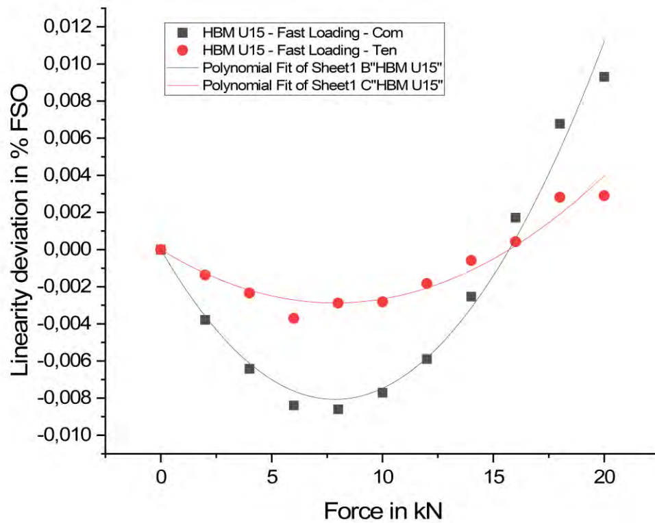
Figure 23 Instantaneous linearity deviation – HBM U15 in tension and compression mode
