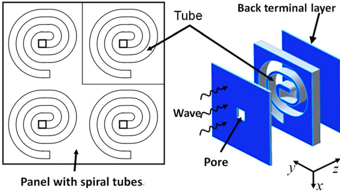
Figure 1: Schematic draw of the sound absorptive panel with spiral tubes [8].
