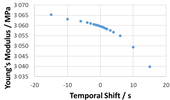
Figure 8: JHS Young's modulus as function of the temporal shift
