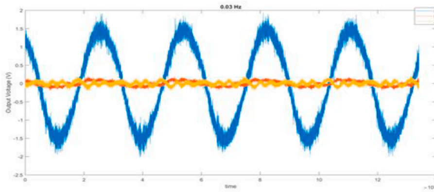
Fig. 6. The contributions of transverse motions.
