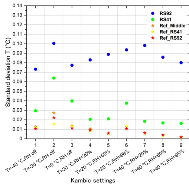
Figure 8. Standard deviations of temperature measurements (vertical axis) from the radiosondes (circles) and the reference thermometers (stars) calculated at the different temperature ( T ) and relative humidity ( RH ) conditions in the Kambic chamber (horizontal axis). At T \leq 0 °C there is no relative humidity control in the chamber ( RH off). The blue and green circles refer to RS92 and RS41, respectively. The red, yellow and orange stars refer to the reference thermometer close to RS92, to RS41 and in the middle of measurement frame, respectively.
