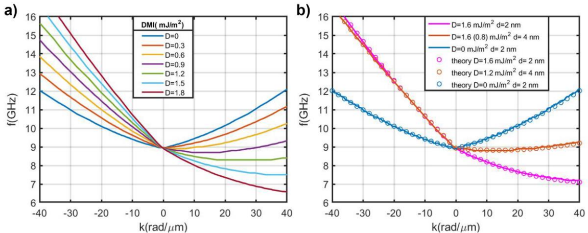
Fig.2 a) Micromagnetic simulations of spin wave dispersion relations in a plain film, 2 nm thick, for different values of the effective DMI constant D . The curves become strongly non-reciprocal with the increasing D . In b) the results of micromagnetic simulations (continuous line) are compared with the analytical expression of the spin waves dispersion relation derived from Eq. 1 (points).
