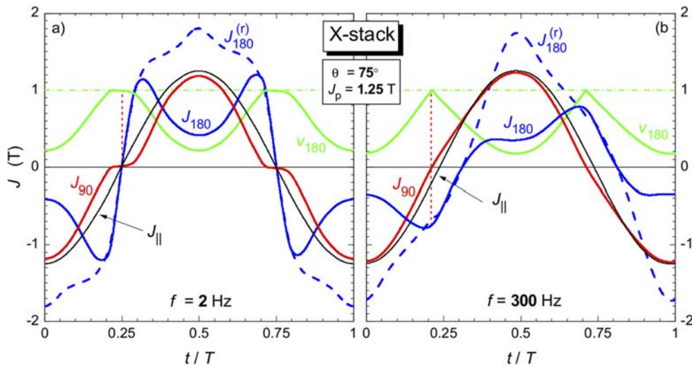
FIG. 5. X-stacked strips cut at \theta = 75^\circ are tested at 2 (a) and 300 Hz (b) ( T = 1/f ) under sinusoidal polarization J_{||}(t) at peak value J_p = 1.25 T. The individual strips are endowed with measurable transverse magnetization J_{\perp}(t) , whose behavior permits one to obtain, via Eqs. (3)–(5), the contributions J_{180}(t) and J_{90}(t) provided by the [001] and [100] [010] phases, respectively, besides their fractional volumes v_{180}(t) and v_{90}(t) ( v_{180}(t) + v_{90}(t) = 1 ). The quantity J_{180}^{(r)}(t) = J_{180}(t)/v_{180}(t) is the polarization value referred to v_{180}(t) . Eddy current fields modify, for a same J_{||}(t) , the relative contribution, phase relationship, and degree of distortion of J_{180}(t) (RD) and J_{90}(t) (TD).
