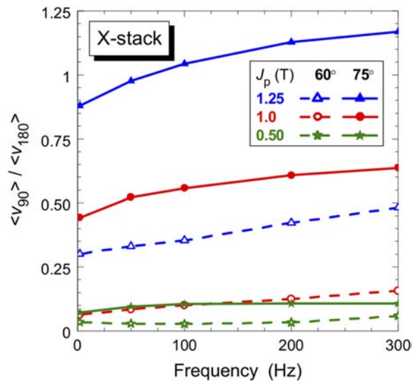
FIG. 6. The period-averaged fractional sample volume ( v_{90} ) ([100] and [010] phases) increases with frequency, for a given J_p , at the expense of ( v_{180} ) ([001] phases). In fact, the eddy currents restrain more effectively the motion of the 180° dws with respect to the 90° dw transitions.
