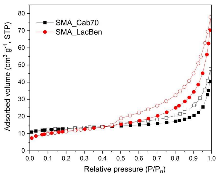
Figure 3. N 2 adsorption-desorption isotherms at 77 K of SMA_Cab70 and SMA_LacBen materials.
