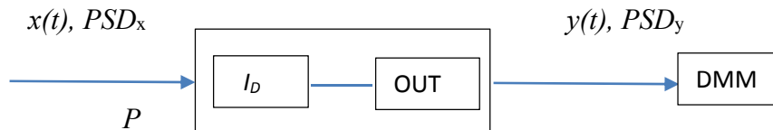
Figure 2. The system of the two instruments: a direct current detector and a DMM connected to its output.
