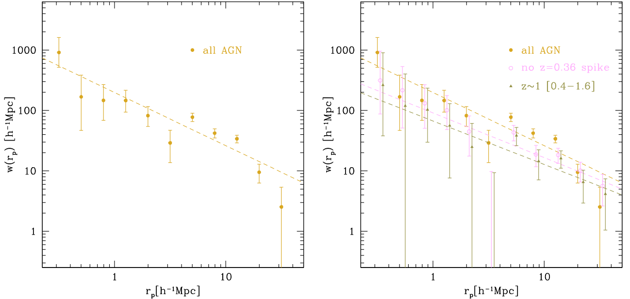
Fig. 6. Left panel: projected correlation function for the XMM-COSMOS AGN reference sample (538 objects with z = 0.2\text{--}3.0 and I_{\text{AB}} < 23 , see Table 1). In this and in the following panel , errors are 1\sigma Poisson confidence intervals and the best-fit power law is shown as a dashed line. Right panel: projected correlation function of the full sample computed including (open circles) and excluding (filled circle) the 42 objects in the large-scale structure at z \sim 0.36 : it is evident that the z \sim 0.36 structure is largely responsible for the signal excess on scales r_p \sim 5\text{--}15\ h^{-1}\text{ Mpc} . The projected correlation function for the z = 0.4\text{--}1.6 sample is also shown (filled triangles). For display purposes, the w(r_p) datapoints of the different samples have been slightly shifted on the r_p axis.
