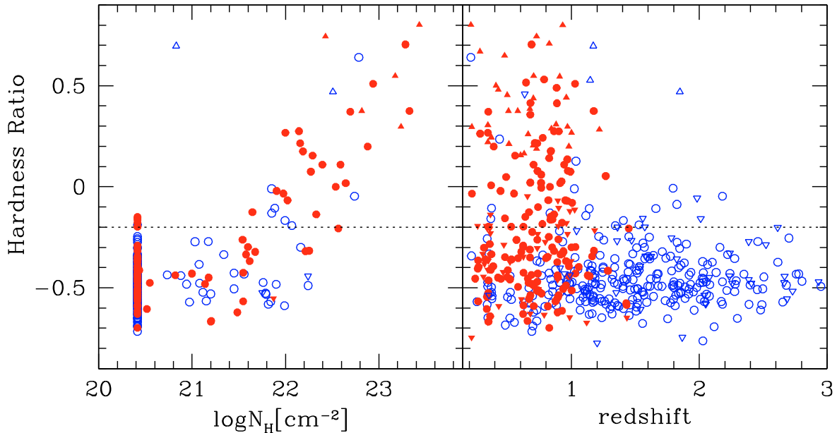
Fig. 8. Left panel. Column density N_H vs. hardness ratio distribution for the 290 objects in our reference sample with more than 200 photons in the 0.5–10 keV band, for which an accurate N_H measurement can be performed through X-ray spectral fitting. Objects that do not show absorption have been plotted at \log N_H = 20.4 , i.e. at the Galactic value. Broad line AGN and non-broad line AGN are shown as blue open and red filled symbols, respectively. Circles refer to objects detected in both soft and hard X-ray bands, for which an HR value is directly measured. Upward (downward) pointing triangles represent lower (upper) limits to the hardness ratios. It is evident that most objects above the dotted line at \text{HR} = -0.2 are absorbed by column densities \log N_H > 21.6 . Right panel. Hardness ratio vs. redshift plot for the 538 sources in our reference sample. Symbols are as in the left panel . The dotted line at \text{HR} = -0.2 marks the adopted dividing line between X-ray absorbed and unabsorbed AGN.
