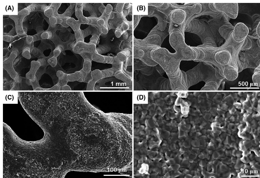
FIGURE 5 SEM micrographs displaying (A and B) the 3D trabecular architecture of hydroxyapatite scaffolds, (C) the trabecular cross-section and (D) a detail of the sintered walls at higher magnification
