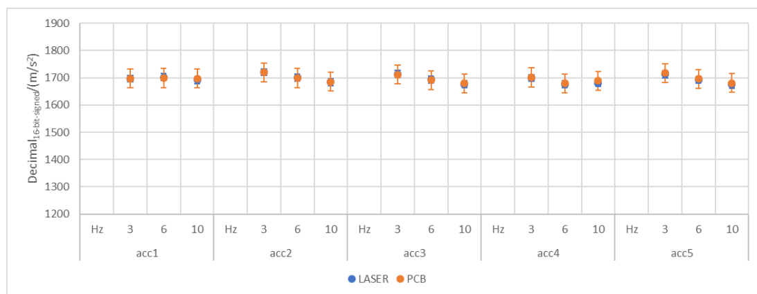
Figure 7. Comparison between sensitivities, obtained using laser and piezoelectric accelerometer as a reference. Processing method: “FFT”. Results for: a) the x-axis; b) the y-axis; c) the z-axis.
