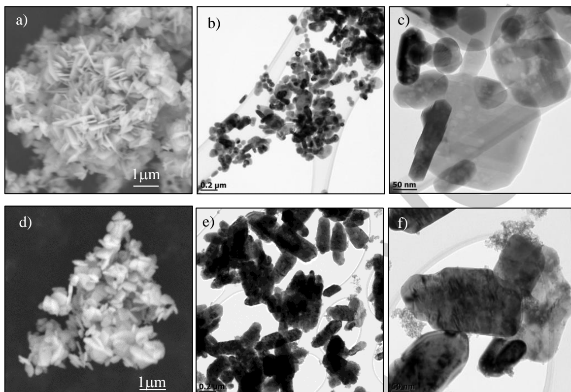
Figure 2. SEM (a, d) and TEM (b, c, e, f) images of ZnO (a, b, c) and Ce-ZnO (d, e, f).
