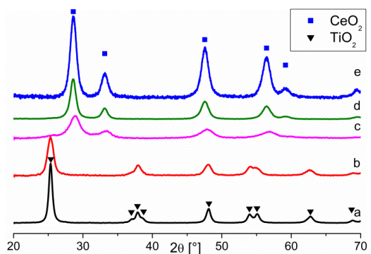
Fig. 1 . XRD of \text{CeO}_2/\text{TiO}_2 mixed oxides: (a) \text{TiO}_2 (sol-gel); (b) 10% mol \text{CeO}_2 , CT10;(c) 50% mol \text{CeO}_2 , CT50; (d) 90% mol \text{CeO}_2 , CT90; (e) \text{CeO}_2
