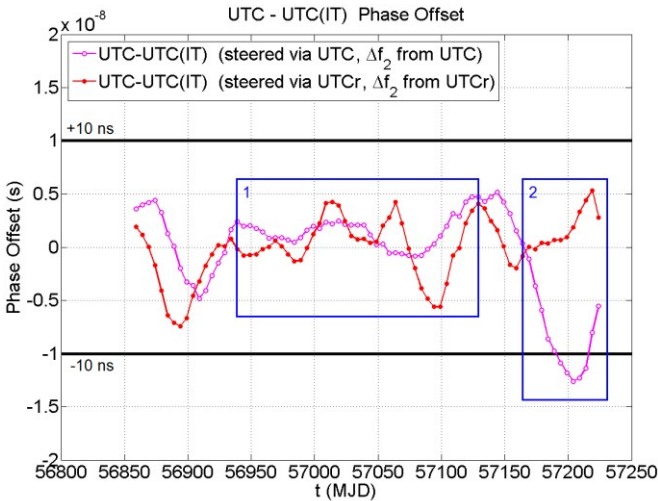
Figure 8. Comparison between the test results for the UTC (purple curve with empty circles) and UTC r (red curve with dots) steering algorithms. The behaviour of the two time scales in the regions highlighted by the blue boxes is described in the text.
