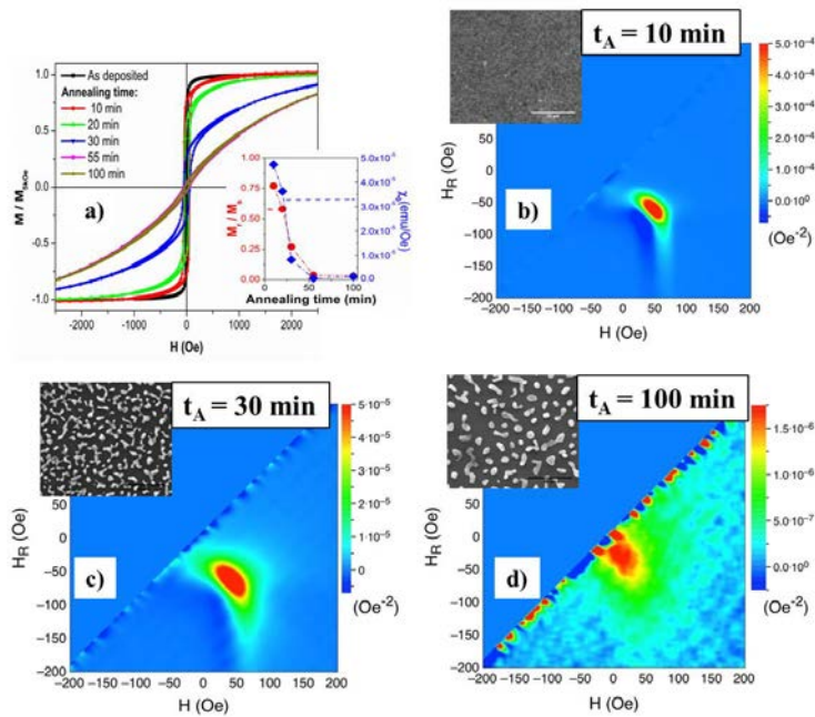
Figure 4. a) Normalized room-temperature hysteresis loops of as-deposited and dewetted samples at T_A = 870^\circ\text{C} for selected t_A , inset: magnetization remanence and coercive susceptibility as a function of t_A ; b) - d) FORCs colour plot of dewetted samples at T_A = 870^\circ\text{C} for selected t_A , inset: SEM image of the corresponding sample.
