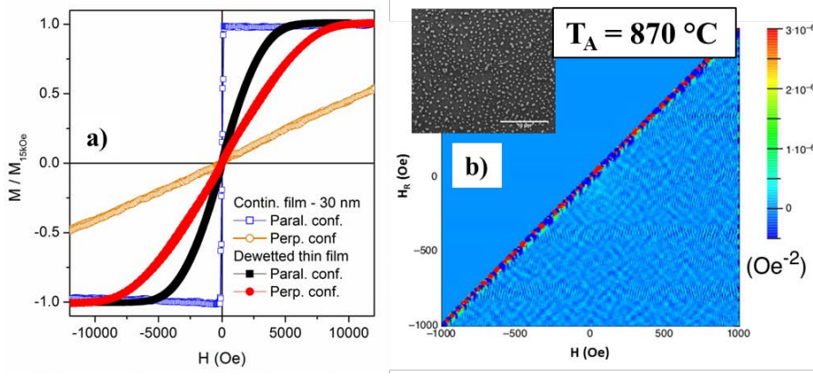
Figure 5. a) normalized room-temperature hysteresis loops of FePd samples ( t = 30 nm) in as-deposited continuous state (blue and orange curve) and after dewetting at T_A = 870 °C for t_A = 55 minutes (red and black curve) measured both in-plane and out-of-plane configuration. b) FORC colour plot of sample dewetted at T_A = 870 °C for t_A = 55 minutes, inset: SEM image of the sample.
