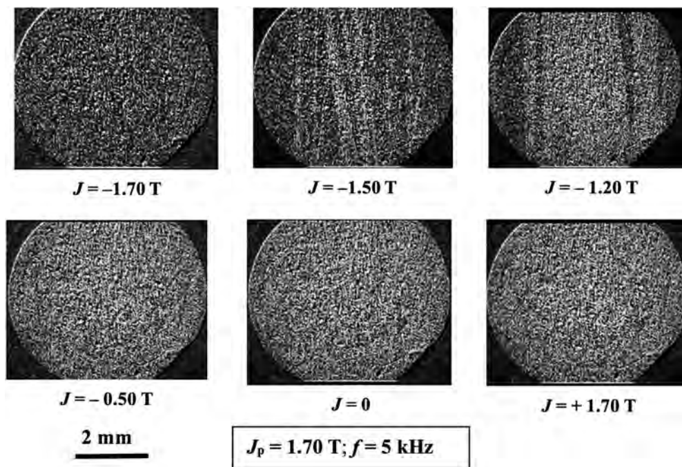
FIG. 5. As in Fig. 4 along an ascending semi-cycle run between -1.70 T to +1.70 T at 5 kHz.
