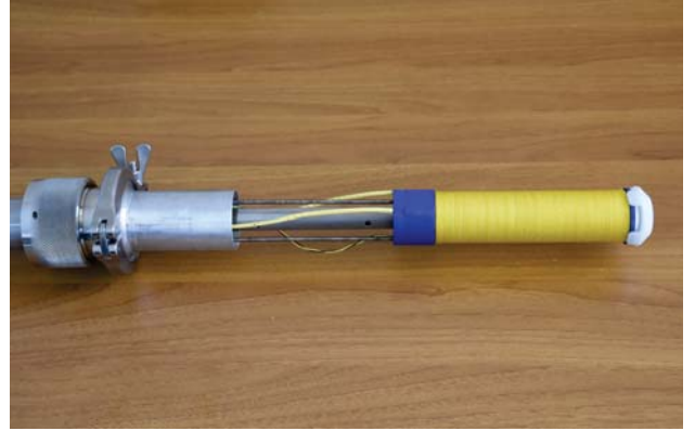
Fig. 2. The probe cryomagnet, showing the yellow winding insulation. A header (white) has been added to ease the insertion in the cryostat.
