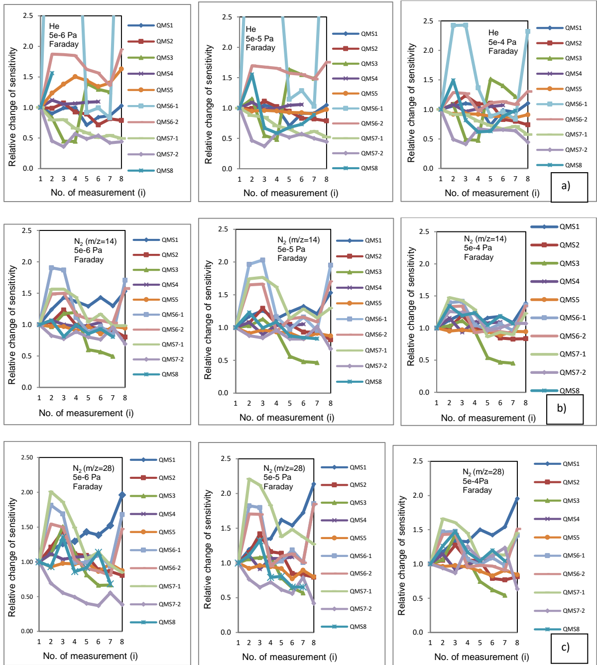
Fig.1 Changes in QMS sensitivity normalized to the initial at 5 \times 10^{-6} Pa, 5 \times 10^{-5} Pa and 5 \times 10^{-4} Pa using only Faraday detector. a) Helium, b) N 2 (m/z=14), and c) N 2 (m/z=28); time interval between each measurement is about three months.
