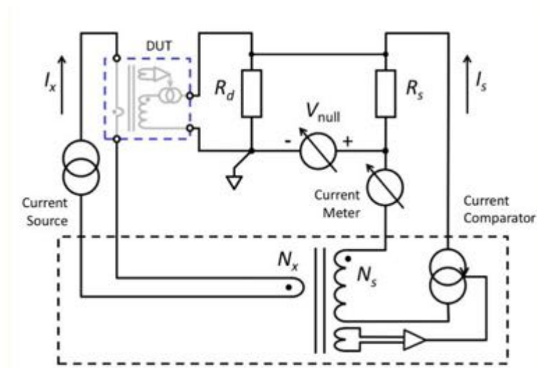
Figure 4. Schematic overview of the adapted low-ohmic measurement bridge at VSL used for DC current ratio measurements. The blue-dashed box at the left top indicates the device under test.
