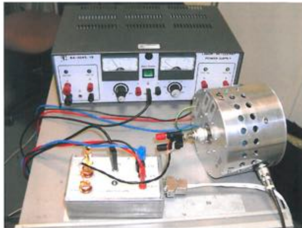
Figure L2: The \pm 15 V power supply, the 1 \Omega resistor and the connection box of the travelling ZFCT.
