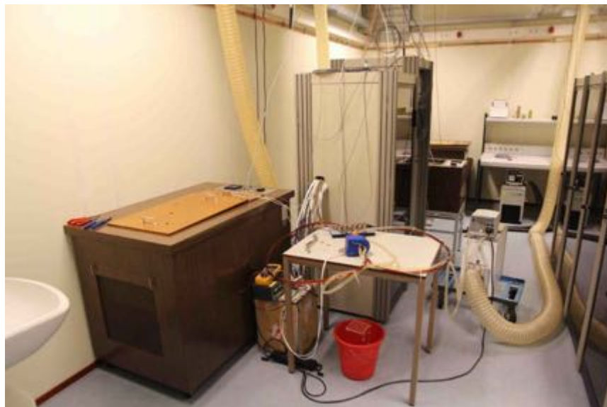
Figure 2. Overview of the VSL measurement setup during the comparison. Measurement rack with low-ohmic resistance bridge (back), water cooling unit (right), oil bath containing R_0 resistors (left) and in the front the unit to be measured, the LEM IT-600 S current transformer, with several primary current loops (on the table in the middle). Note the two tubings which removed the heat from the oil bath and water cooling unit respectively, in order to minimise the heat load of the measurement room.
