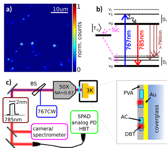
Figure 1. a) Wide-field (WF) fluorescence image: zoom ( 40 \times 40 \mu\text{m}^2 ) on a region of the sample showing bright nanocrystals. b) Blue-detuned (767 nm) pumping scheme used to collect photons emitted into the 00-ZPL (785 nm). In order to properly model the molecule photo-physics, the metastable triplet state should be taken into account. Fluorescence is inhibited when the molecule is in its triplet state, which is hence responsible for blinking. However, this state is very unlikely populated in the case of DBT in Ac, with a probability (namely inter system crossing yield) ISC < 10^{-5} . c) Simplified sketch of the optical setup used for the measurement reported in the paper (details are presented in Section 6) and sketch of the device operated as single-photon source. Au, gold; AC, anthracene; DBT, dibenzoterrylene; PVA, polyvinyl alcohol.
