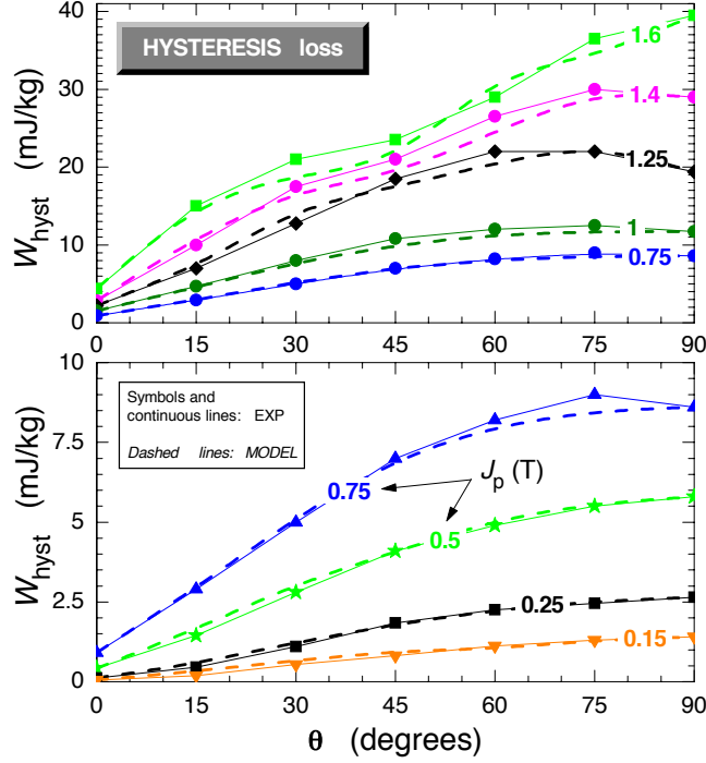
Figure 5: Behaviour of the hysteresis loss component vs. the cutting angle \theta formed by the applied field with RD (see Fig. 1), for high (top) and low (bottom) peak polarisations J_p . The theoretical loss figures at intermediate ( 15^\circ \leq \theta \leq 75^\circ ) cutting angles are obtained after interpolation performed via Eq. (6) of the RD and TD experimental values.
