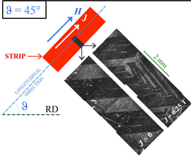
Figure 3: Surface domain structures, obtained by Kerr microscopy, of a strip cut with its longitudinal direction making an angle \theta = 45^\circ to RD. Two situations, corresponding to the demagnetised state and J = 0.25T , are reported.
