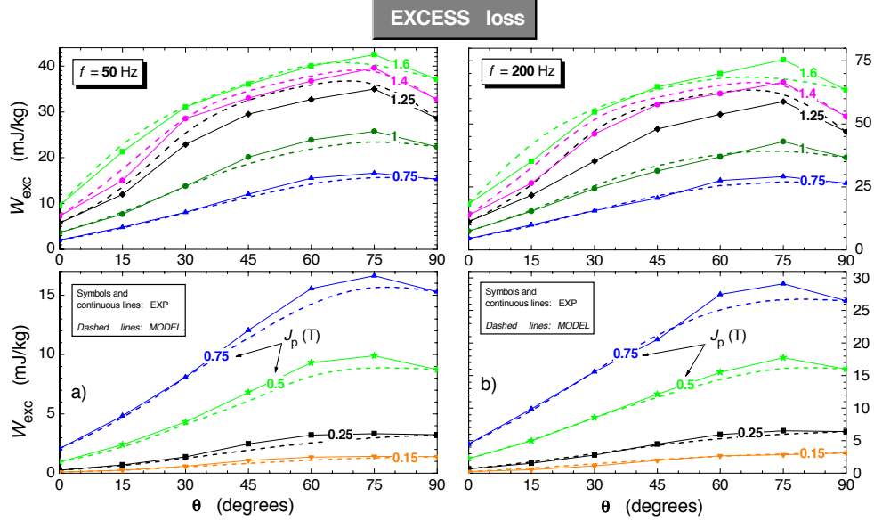
Figure 6: Behaviour of the excess loss component vs. the cutting angle \theta formed by the applied field with RD (see Fig. 1), for low (bottom section) and high (top section) peak polarisations J_p , at f = 50 Hz (a) and f = 200 Hz (b). The theoretical loss figures at intermediate ( 15^\circ \leq \theta \leq 75^\circ ) cutting angles are obtained after interpolation performed via Eq. (9) of the RD and TD experimental values.
