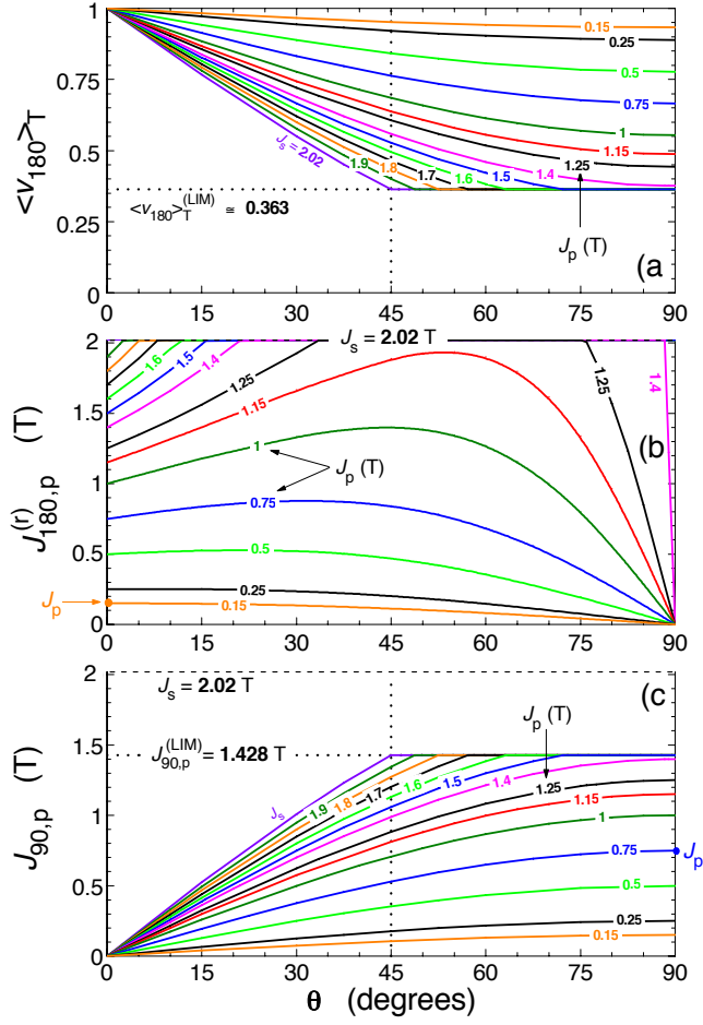
Figure A.1: Behaviour, vs. the angle \theta formed by the applied field with RD, of the model parameters \langle v_{180} \rangle_T , limited by the lower threshold \langle v_{180} \rangle_T^{(LIM)} (a), J_{180,p}^{(r)} (b), and J_{90,p} , limited by the upper threshold J_{90,p}^{(LIM)} (c).
