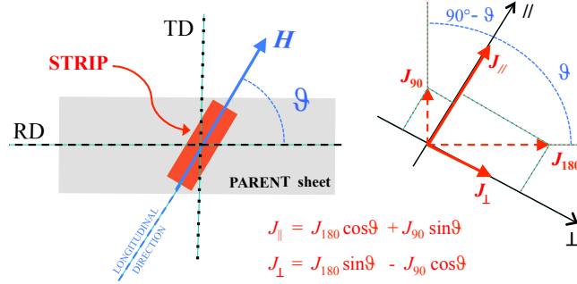
Figure 1: Left side) The strips used in the experiments are cut in such a way that the specimen longitudinal direction, along which the magnetising field \mathbf{H} is applied and the induction revealed, forms an angle \theta with the parent sheet rolling direction (RD). The transverse direction (TD) is also indicated. Right side) The measured \mathbf{J}_{\parallel} and \mathbf{J}_{\perp} (solid arrows), together with the polarisations (referred to the whole sample volume) \mathbf{J}_{180} and \mathbf{J}_{90} , generated by the 180^\circ and 90^\circ phases (dashed arrows), are depicted [see Eqs. (A.1)].
