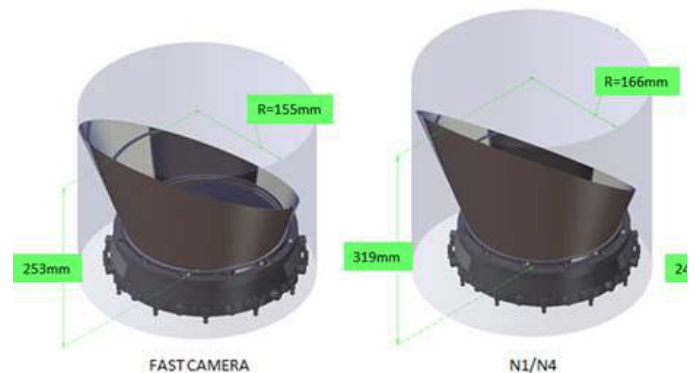
Fig. 1. Two out of the three kind of baffles to be used on the PLATO mission cameras.
