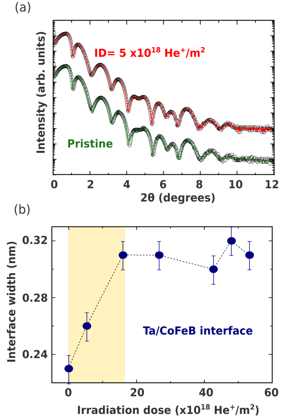
FIG. 3: (a) X-ray reflectivity profiles for a pristine and an irradiated film at ID = 5 \times 10^{18} \text{ He}^+/\text{m}^2 , the corresponding model is plotted as solid lines. (b) Width of the Ta/CoFeB interface as a function of the irradiation dose.
