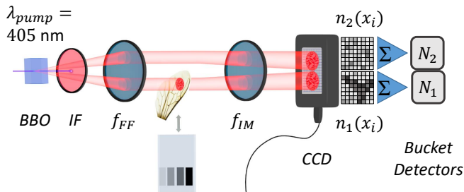
FIG. 5: Scheme of the experimental set-up. In the BBO crystal two beams with perfect correlation in the photon number (twin-beam state) are generated. The probe beam interacts with the sample and is detected by a half of a CCD camera chip, while the other beam goes directly to the second half of the chip. The equivalent bucket detector on both channels are simulated by integrating (summing pixels signal) over the two regions. Two different samples are used: a set of uniform depositions of different transmittance t_- and a biological object, i.e. a wasp wing.
