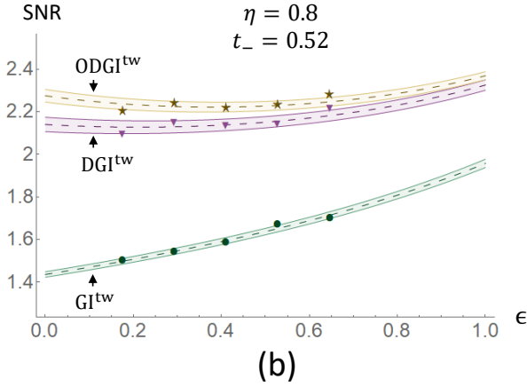
FIG. 6: SNR in function of \epsilon , the fraction of the detection area occupied by the deposition, for (a) t_- = 0 and (b) t_- = 0.52 . Green color refers to GI, purple to DGI and yellow to ODGI. The dots are the experimental data, obtained for H \sim 3 \cdot 10^4 frames and an area of \mathcal{N} = 952 pixels. The dashed lines are obtained fitting the data with the theoretical model, considering \eta as free parameter. The confidence region at 1\sigma is also reported as colored bands around the curves.
