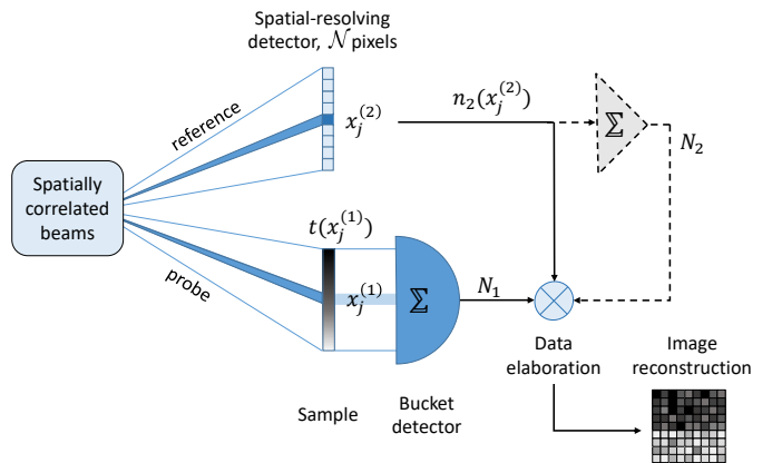
FIG. 1: Scheme of GI and DGI protocols. Spatial correlations between two beams are exploited. The reference beam is detected by a spatial resolving detector, the probe beam, after interacting with the sample impinges on a detector without spatial resolution. Every pixel x_j^{(2)} is in one-to-one correspondence with a resolution cell x_j^{(1)} at the object plane. For the image reconstruction the number of photons detected by the bucket detector N_1 and the one detected by each pixel in the resolving detector, n_2(x_j^{(2)}) , are used in the data elaboration. In DGI protocol (dashed path) also the integrated signal N_2 is exploited.
