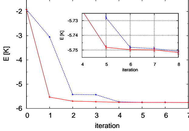
Figure 1: (color online) Convergence of the VMC total energy of N = 64 ^4\text{He} atoms at equilibrium density during the optimization of the Jastrow-McMillan factor with (solid) and without (dashed) regularization.
