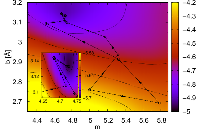
Figure 2: (color online) Convergence of the Jastrow-McMillan factor of N = 64 ^4\text{He} atoms at equilibrium density with (solid arrows) and without (dashed arrows) regularization. To show the improvement brought by the regularization, the flows in the parameter space impressed by the two algorithms are superposed to a contour plot of the energy landscape \mathcal{E}(\mathbf{p}) obtained via several VMC calculations; dotted lines represent level curves of the energy landscape.
