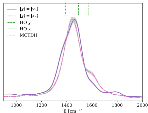
FIG. 5. Semiclassical power spectra in the shared proton perpendicular mode region, employing symmetrized reference states of type (iv) and multireference trajectory sampling, as explained in Sec. III D. The straight dashed lines correspond to the nondegenerate harmonic frequencies of the 8th and 9th normal modes. The dotted line indicates the MCTDH result from Ref. 44. Gray bands behind the curves indicate the standard deviation of the estimated spectra.
