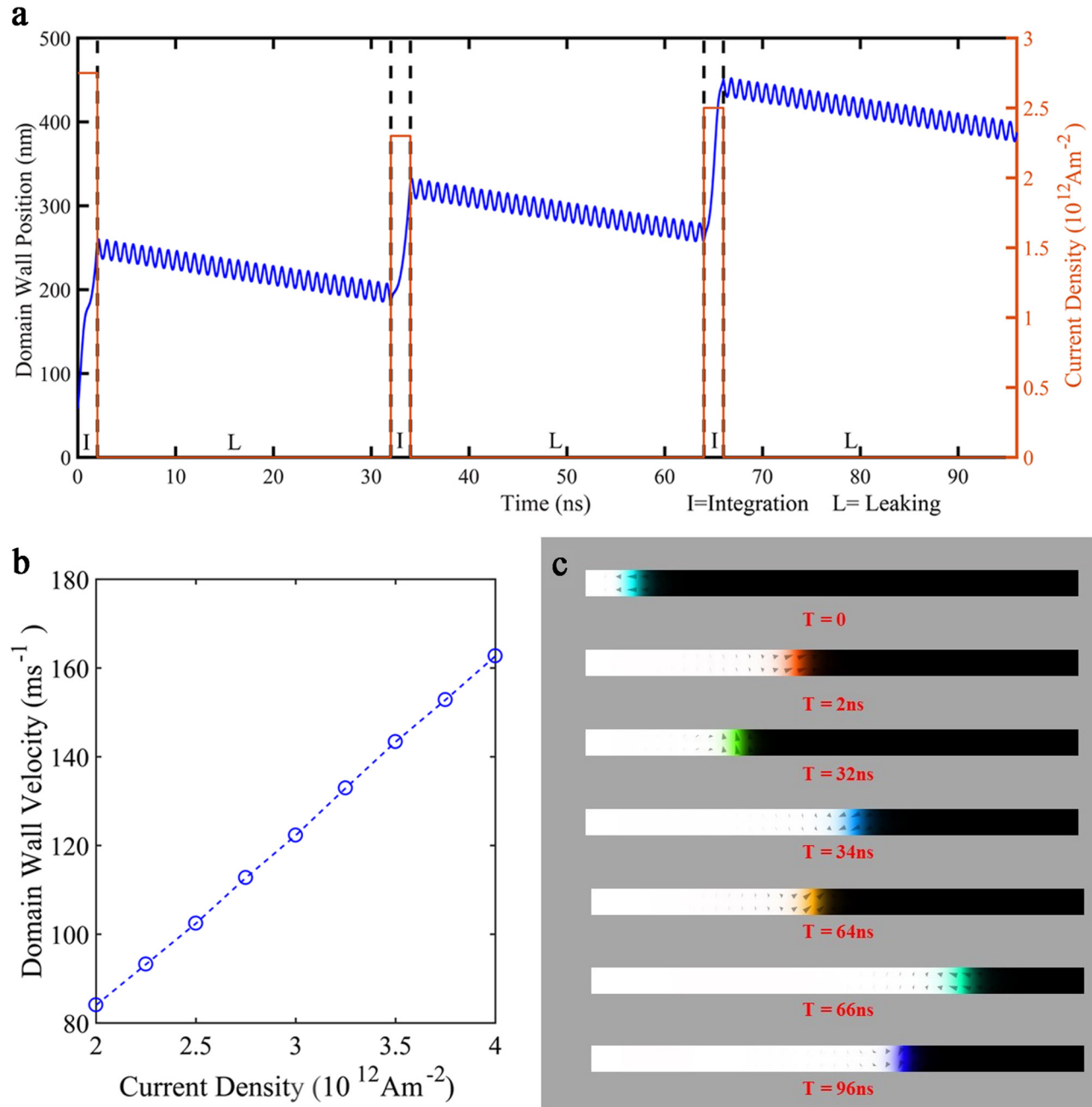
FIG. 4. Leaking and integration of the DW-MTJ neuron. (a) Time vs. DW position plot for three consecutive 2 ns long current pulses of magnitude 2.75 , 2.3 , and 2.5 \times 10^{12} \text{ A/m}^2 , respectively, separated by 30 ns leaking periods. During the current pulse periods, integration functionality is taking place. The leaking functionality resulting from the magnetic field created by the fixed ferromagnet causes precessional DW motion. (b) Current density vs. DW velocity. (c) Mumax3 snapshots of the integration and leaking at the times noted by dashes in the plot of (a). (Multimedia view).
