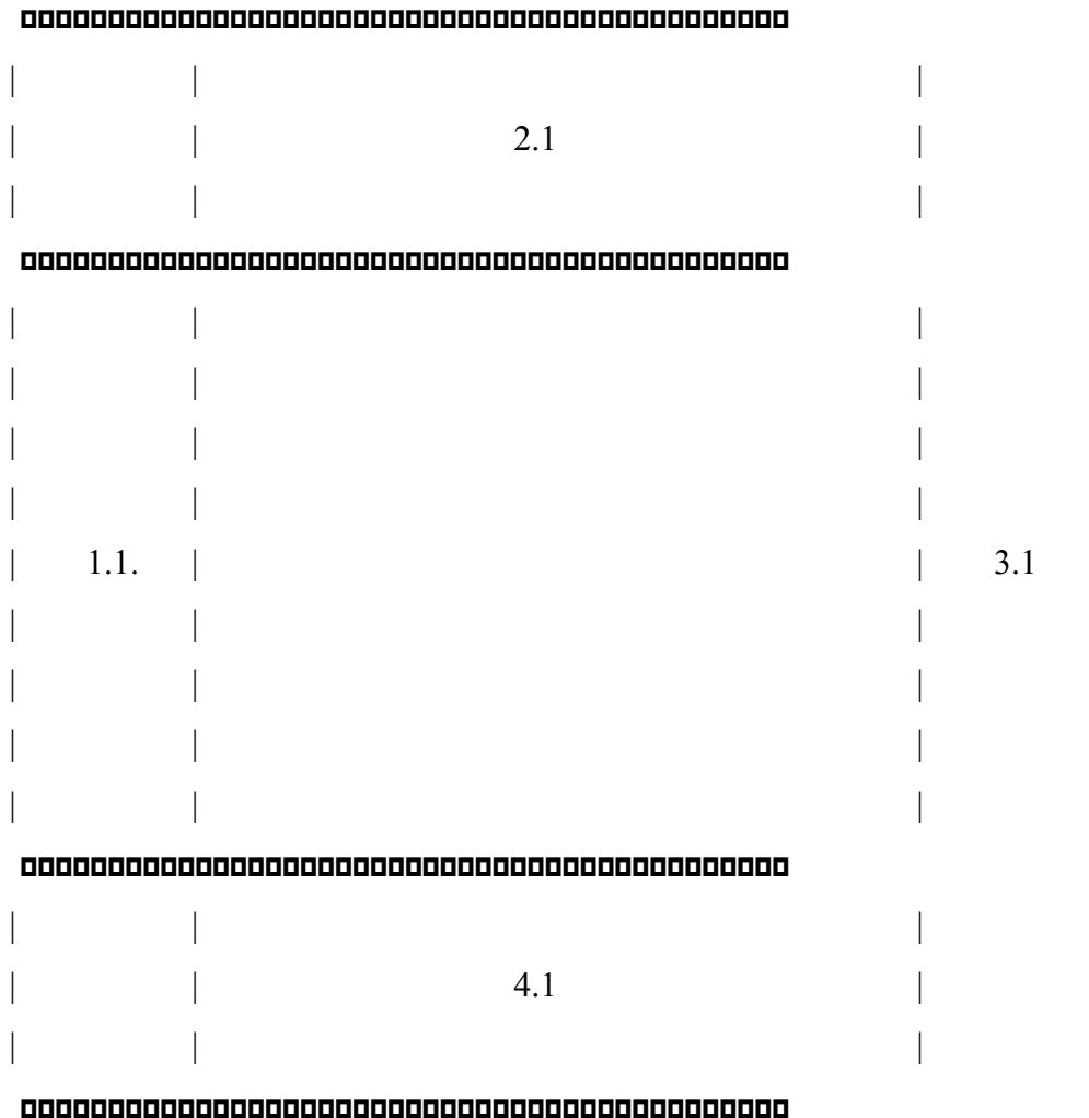
Figure 1 – Method of loading strips in the Epstein frame.
