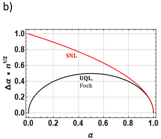
Figure 1. Loss estimation. (a) The loss estimation is obtained by comparing the number of photons detected with and without the absorbing sample. (b) Uncertainty in function of the loss parameter \alpha . SNL stands for shot-noise limit, while UQL stands for ultimate quantum limit.
