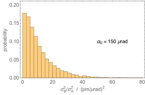
Figure 8. Histogram of 10^4 Monte Carlo calculations of the \sigma_\phi^2/\sigma_\alpha^2 ratio for 150 \mu\text{rad} wavefront misalignment. The jitter is isotropic and has \sigma_\alpha^2 variance. The detector radius is r_0 = 1.1 mm, the normalized radius of the interference pattern is w/r_0 = 1 . The phase profiles \varpi(x, y) are constrained to a \lambda/20 flatness.
