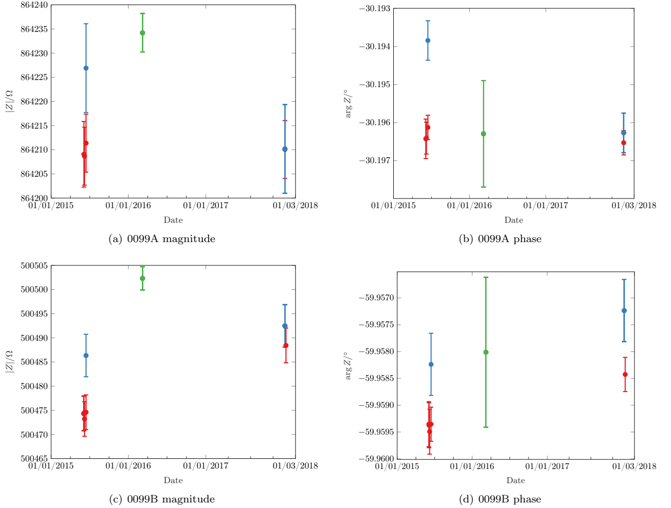
Figure 10. Results for the RC standards 0099A and 0099B: — INRIM 2TP-FD; — INRIM 4TP-DA; — METAS 4TP-FD. Uncertainty bars correspond to a coverage factor k = 2 .
