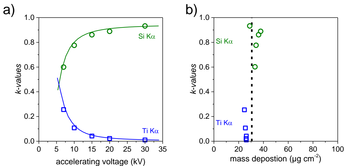
Figure 4: a) k -values of the Si K\alpha and Ti K\alpha vs. applied accelerating voltage, b) k -values versus calculated film mass deposition. Based on experimental k -values, theoretical k -values are iteratively calculated with elemental composition and mass deposition as free parameters (lines in a) so that the mean mass deposition of the \text{TiO}_2 training film can be finally extracted (see dashed line in b).
