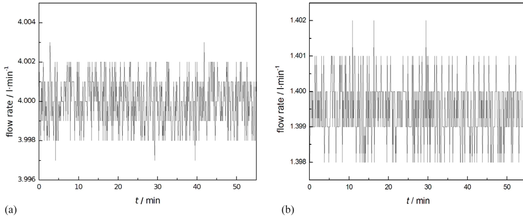
Figure 5. Flow rate stability under the following nominal conditions: (a) T_{\text{bath}} = -94\text{ }^{\circ}\text{C} , \phi = 4\text{ l min}^{-1} and P = 1100\text{ hPa} . Peak-to-peak amplitude = 0.006\text{ l min}^{-1} , mean value = 3.999\text{ l min}^{-1} , standard deviation = 0.001\text{ l min}^{-1} . (b) T_{\text{bath}} = -99\text{ }^{\circ}\text{C} , \phi = 1.4\text{ l min}^{-1} and P = 200\text{ hPa} . Peak-to-peak amplitude = 0.004\text{ l min}^{-1} , mean value = 1.400\text{ l min}^{-1} , standard deviation = 0.001\text{ l min}^{-1} .
