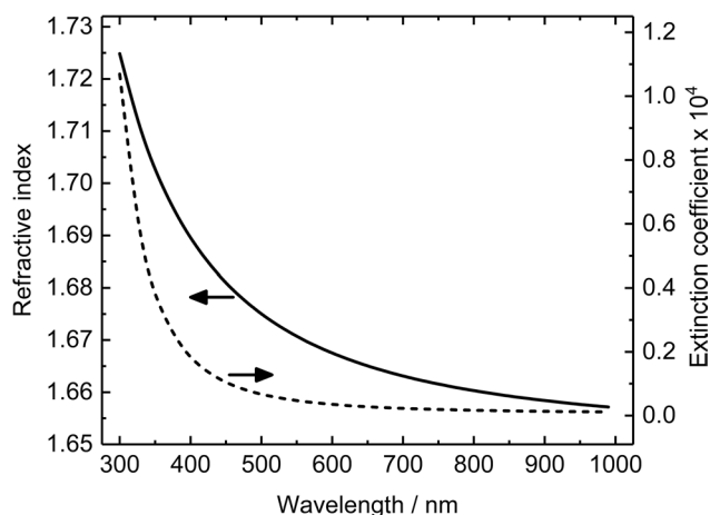
Figure 4. Refractive index and extinction coefficient of the ALD grown \text{Al}_2\text{O}_3 layer of the n -type PQED photodiode.
