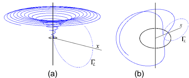
Fig. 3. Flux lines obtained starting at (0.25, 0, 0) m and (0.6, 0, 0) m.
