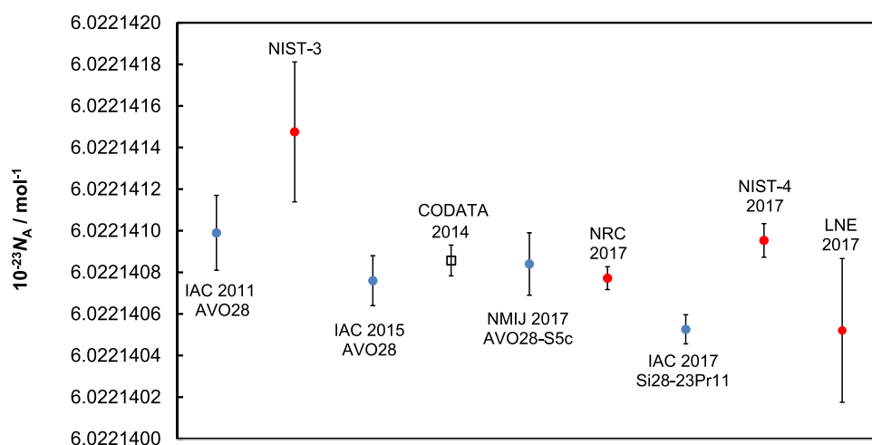
Figure 16. Avogadro constant determinations: comparison between the most accurate N_A values at present available. Bars represent the standard uncertainty.
