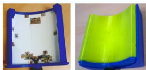
Fig.3: Double-tuned 1H/23Na planar antenna polylactide (PLA) thermoplastic mechanic support
